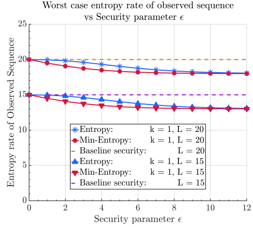
Fig. 7. Entropy rate for worst case access sequence for L = 20 and 15 and k = 1 .
